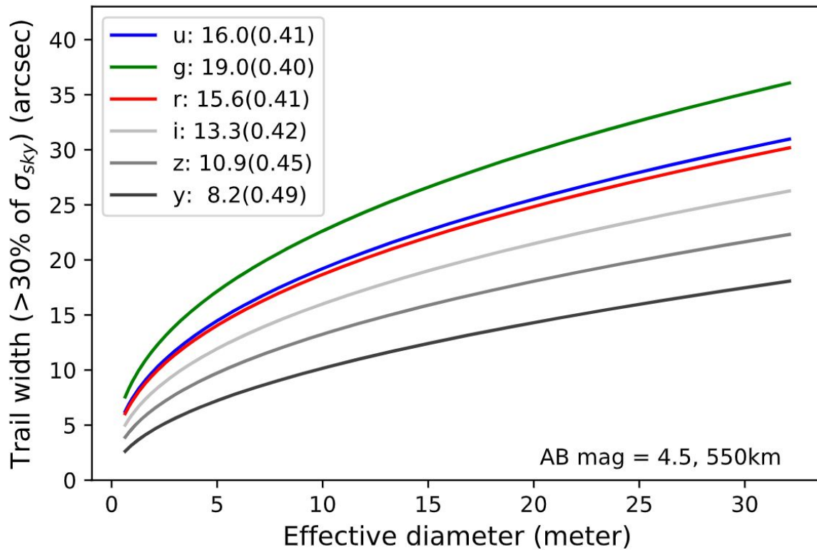
Figure C.10. LEOsat trail width for a 4.5 V_{\text{mag}} satellite vs telescope aperture. Most long exposure spectra would be polluted by even lower surface brightness trails than 30% of sky noise. At 1% sky noise, the trail widths approach 60 arcseconds.
